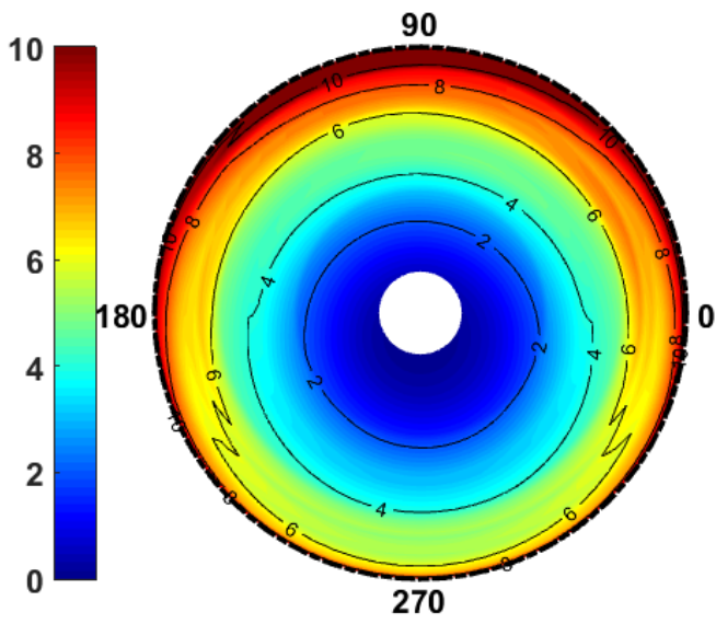
(c) Elemental Profile Drag (lbs/ft), R_{span} = 26.8 ft
