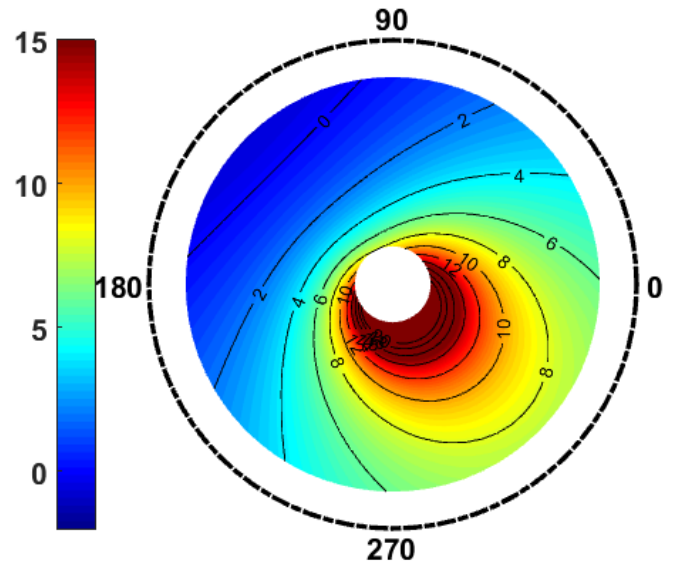
(b) Elemental Inflow Angle (deg), R_{span} = 22.8 ft
