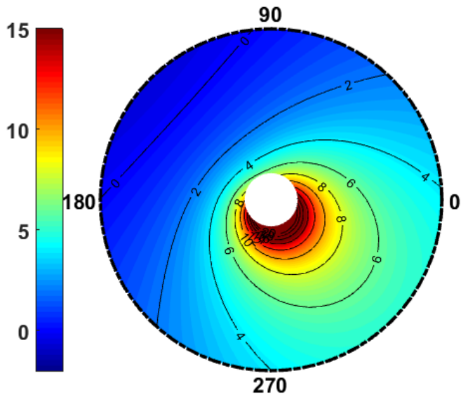
(a) Elemental Inflow Angle (deg), R_{span} = 26.8 ft
