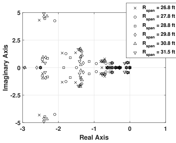
(b) Closed-loop eigenvalues - 40 knots extension
