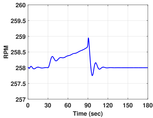
Fig. 15: 40 knots retraction - RPM
