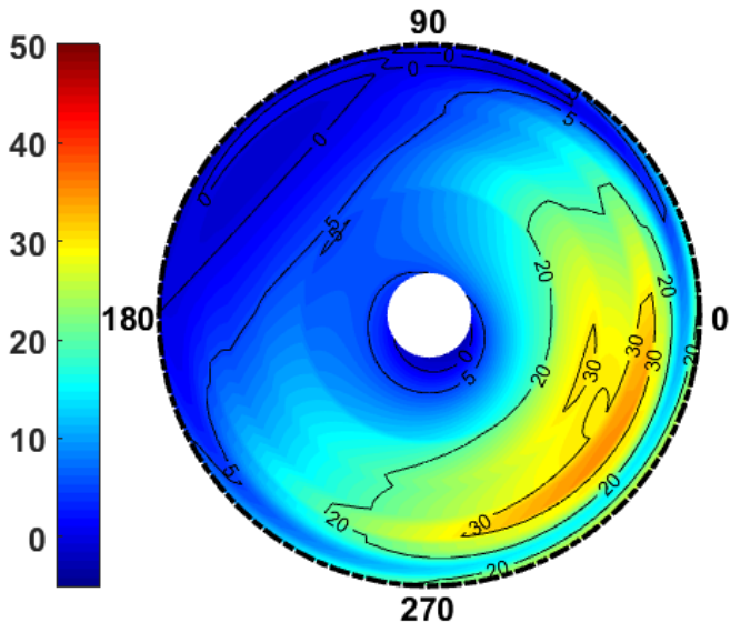
(a) Elemental Induced Drag (lbs/ft), R_{span} = 26.8 ft
