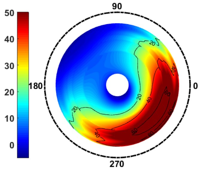
(b) Elemental Induced Drag (lbs/ft), R_{span} = 22.8 ft
