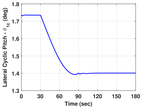
(c) Lateral Cyclic Pitch
